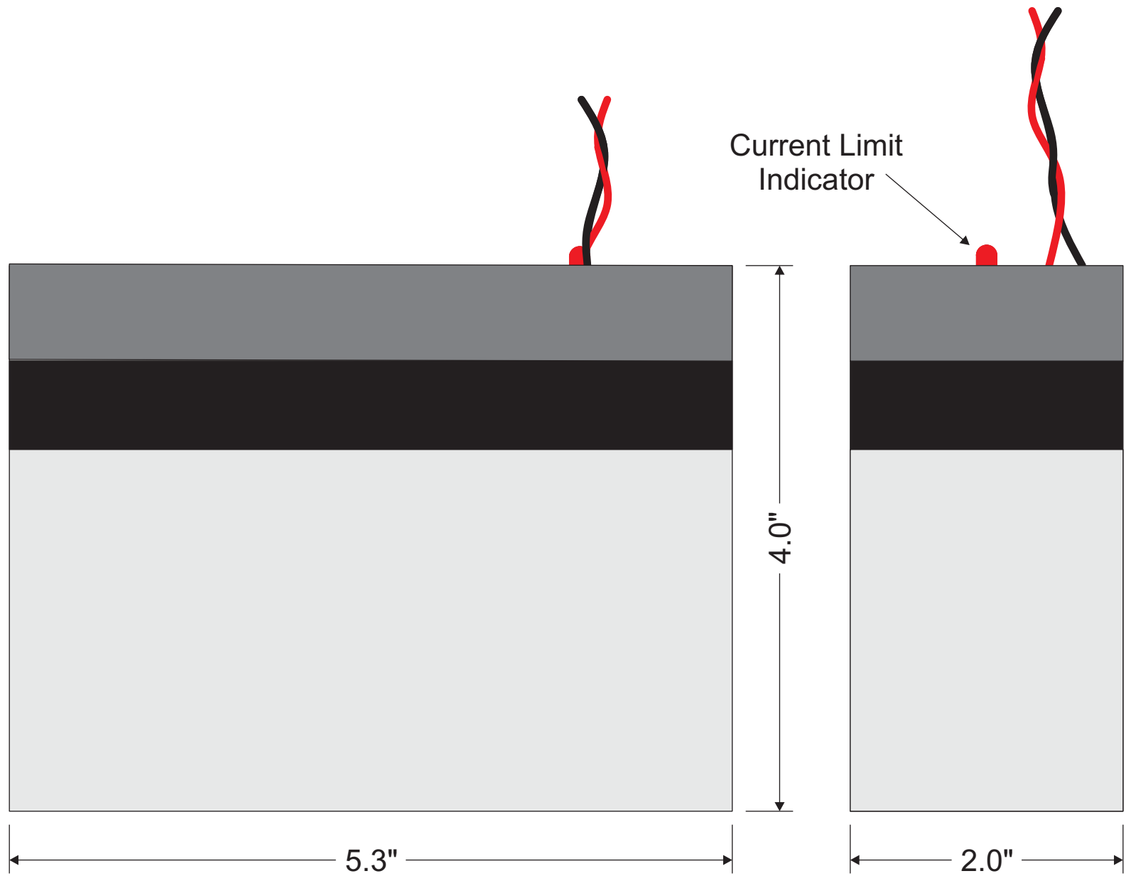
Model BAT-6V-12-IS
